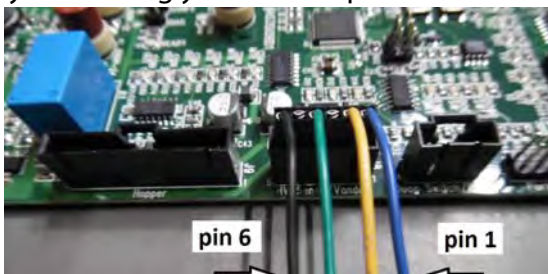
Figure 14. SIO Board - Vandalism Sensor Location
