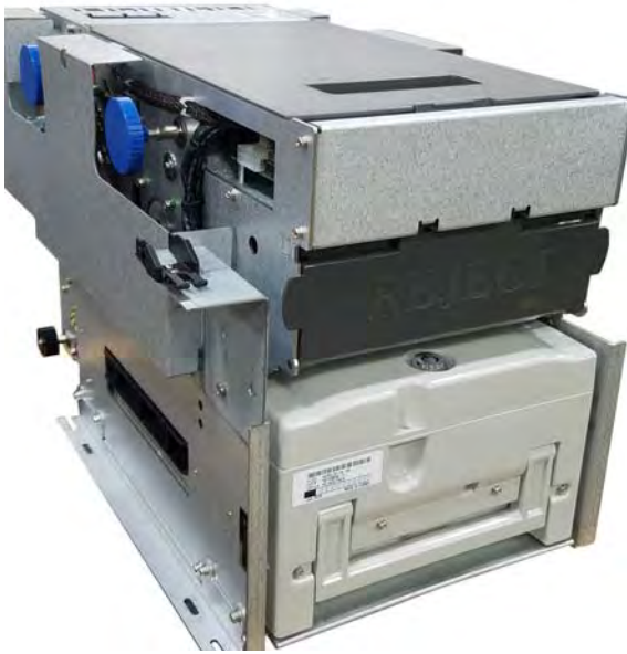
Figure 6. Gen-Mega Bill Dispenser for the Auto Sentry CPT
